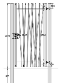
Micmac swing gate
