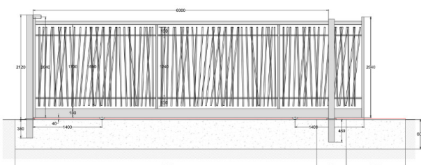
Micmac sliding double gate
